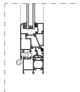
DETAIL 04
