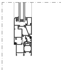
DETAIL 02
