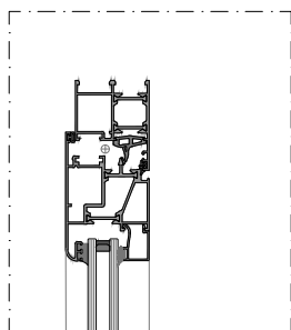
DETAIL 01
