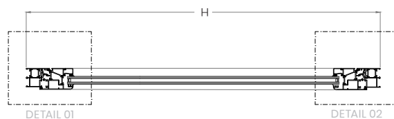
SECTION S1
