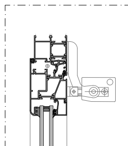
DETAIL 03
